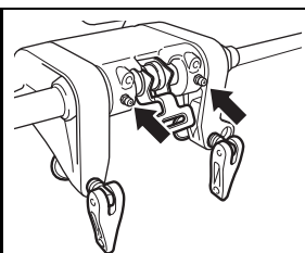
Swivel bracket
