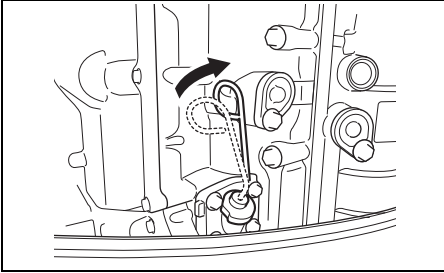
Fuel line
