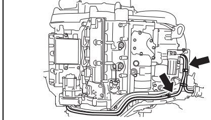
Fuel line
